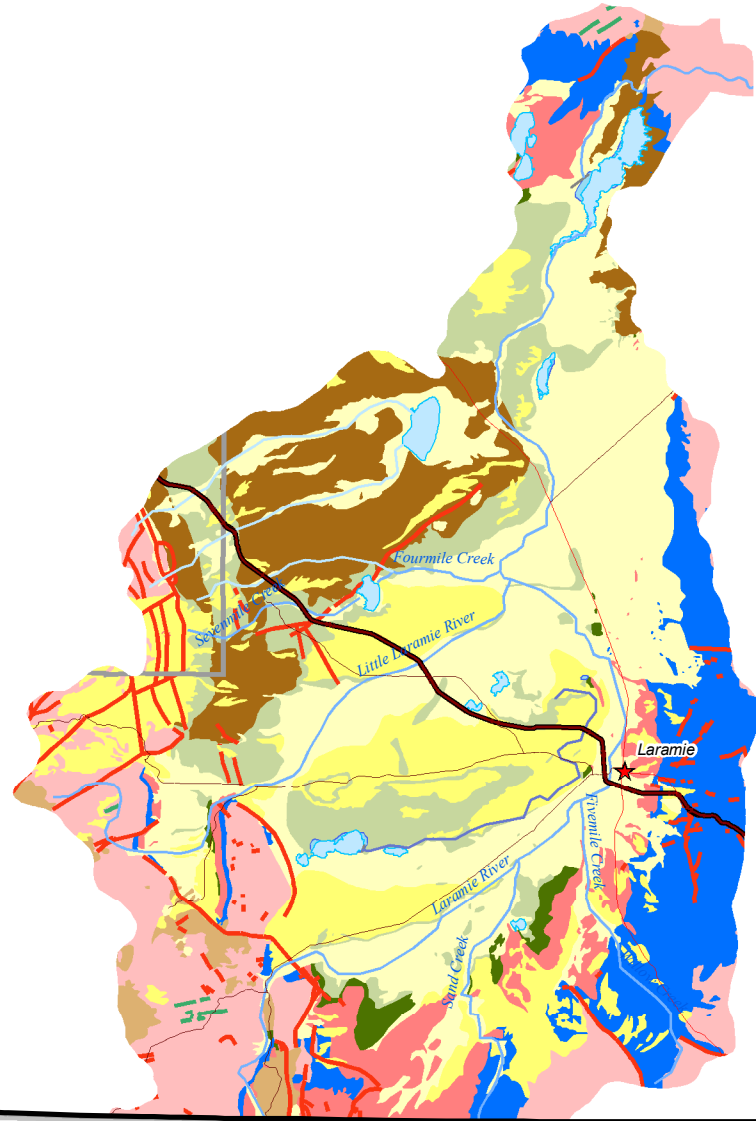
Platte River Basin Water Plan Aquifer Systems Upper Laramie Subbasin
