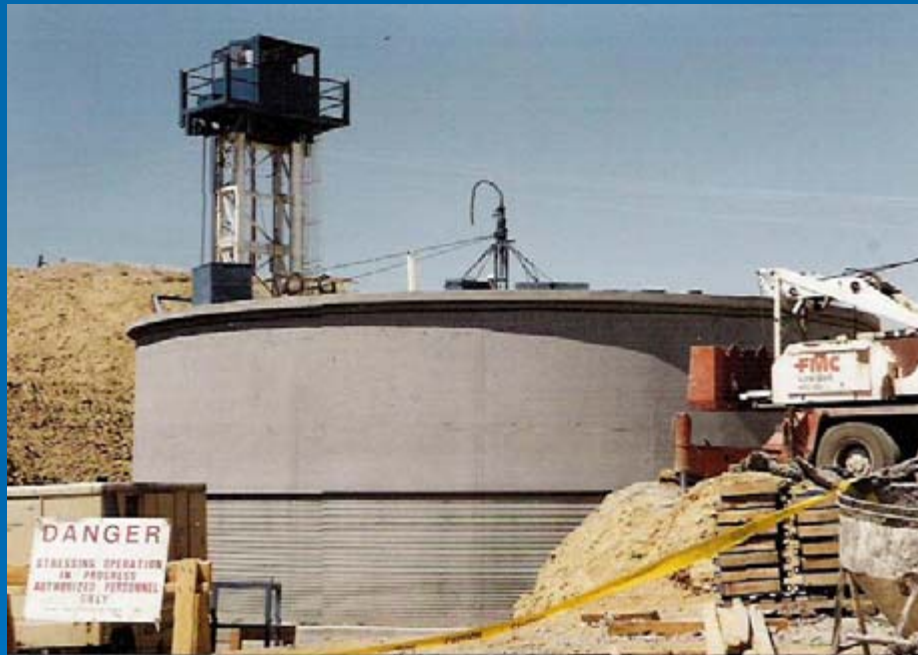
WIRE WRAPPING THE DEAYER TANK
